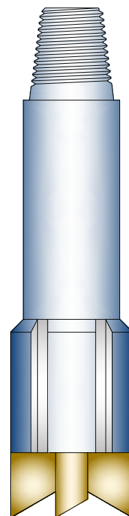
Bladed Junk Mill
